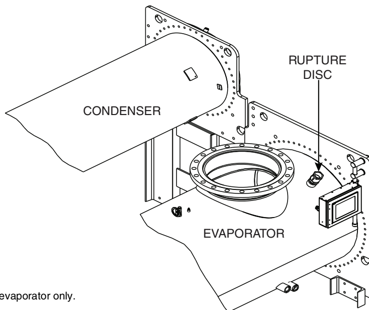
Fig. 17 — Relief Device Arrangements
