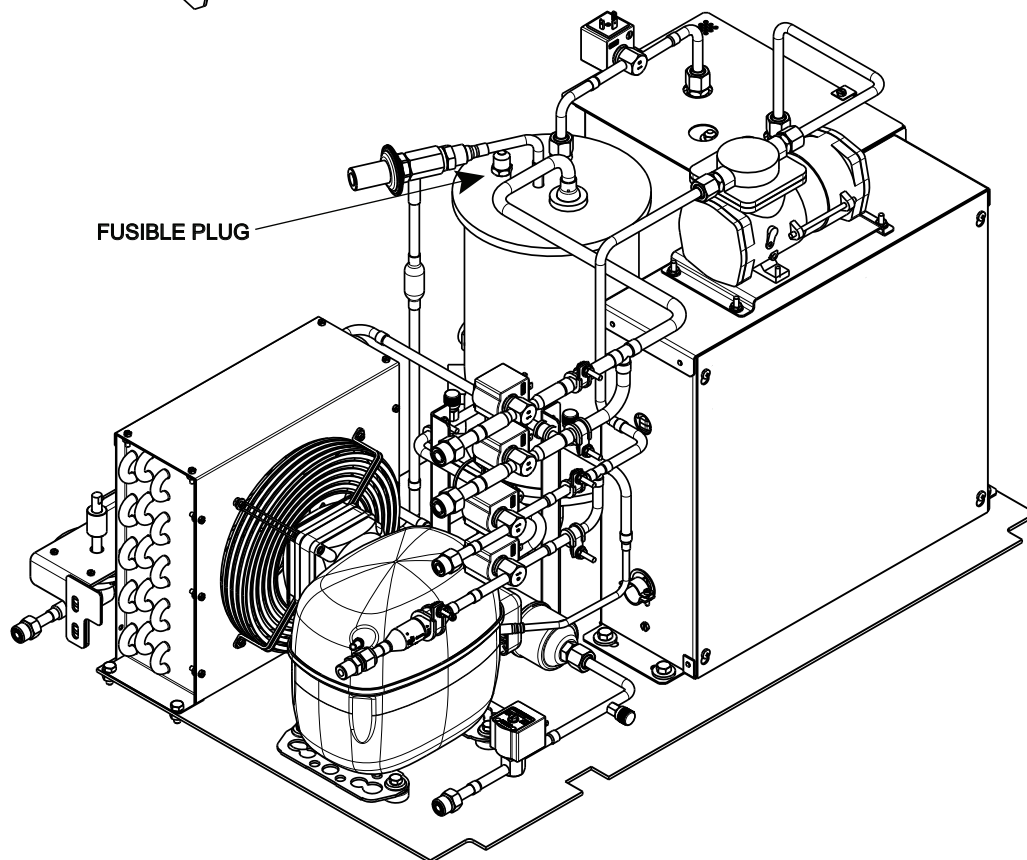
Fig. 10 — Location of Fusible Plugs in Lubrication Assembly and Purge Assembly
