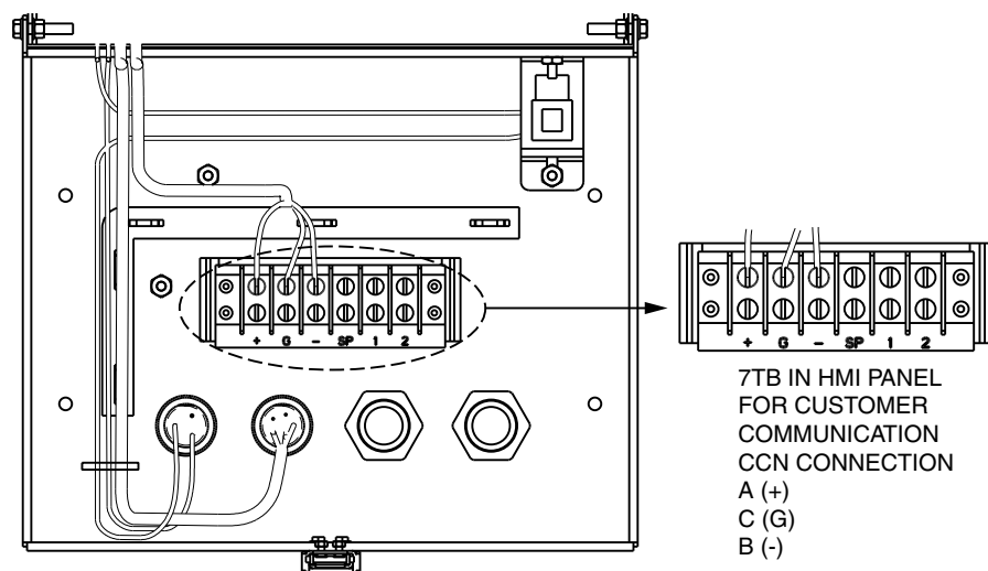
Fig. 20 — HMI Panel
