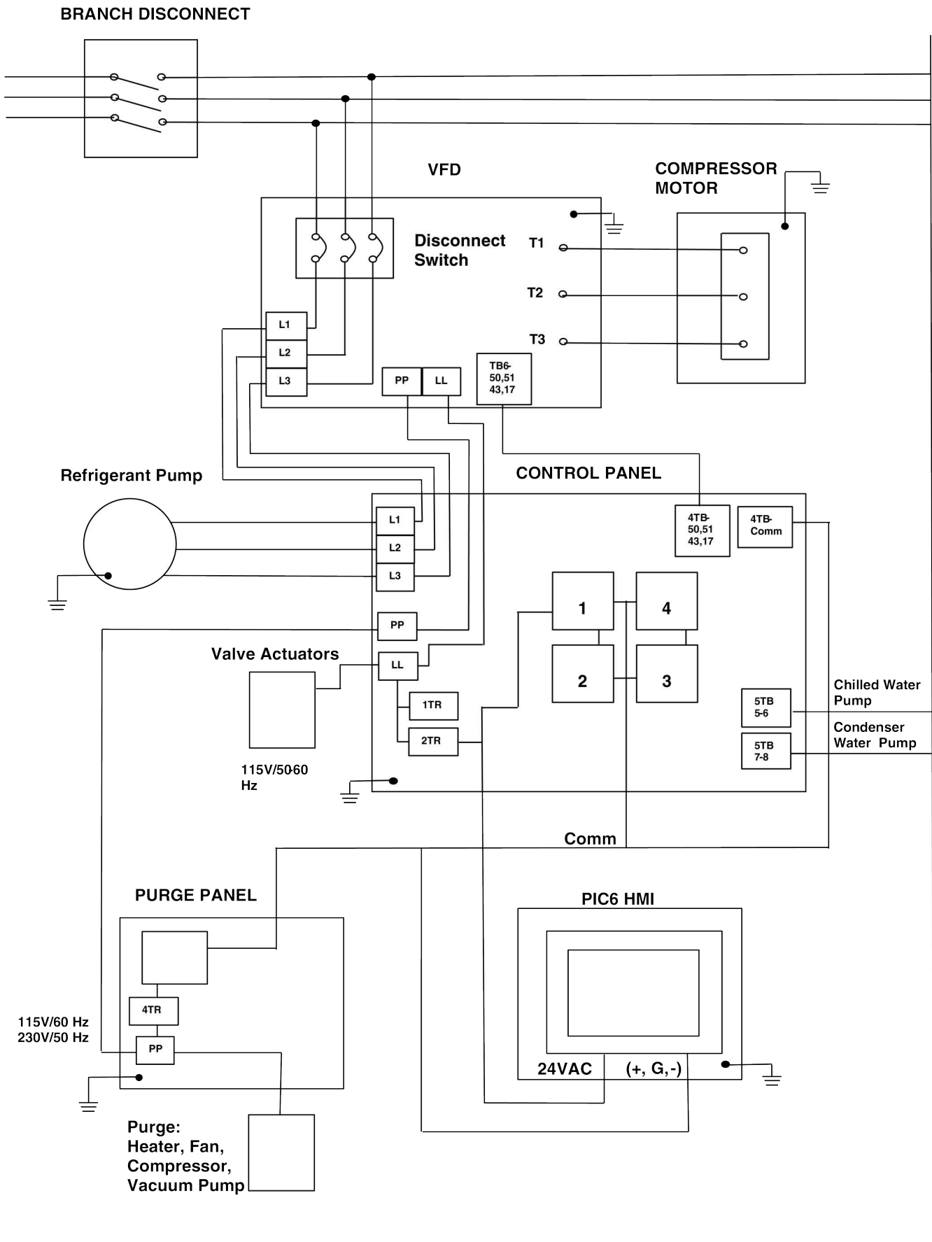
Fig. 27 — Typical 19DV VFD - Factory Unit Mounted
